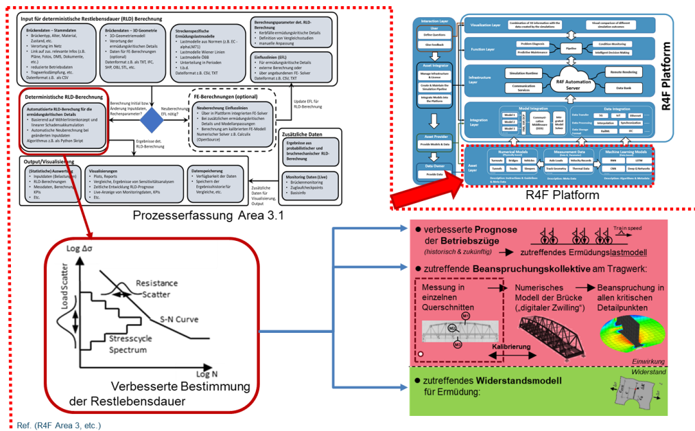
Fig. 2. RLD Model
